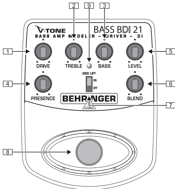
Control elements
